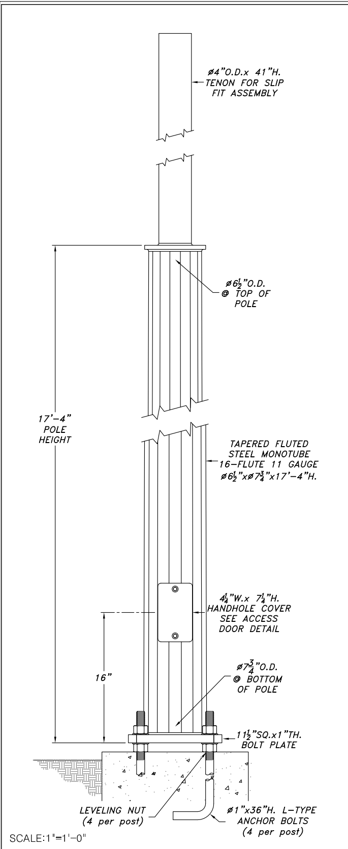
Steel Series-11.5" Bolt Plate-Tapered Fluted Steel Pole-17'-4" Height SS-11.5-TSS-17.33
